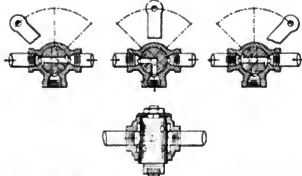
Figs. 1795-1798. Three-Way Cock for Player Traction Increase. Atchison, Topeka & Santa Fe.
